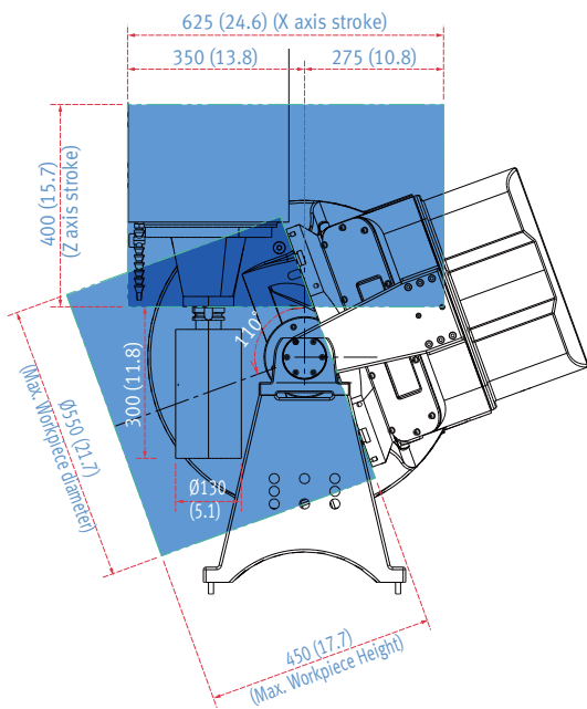
Front view (1:10)
