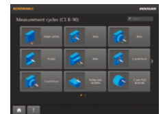
PC software
